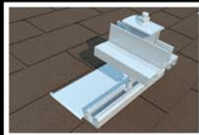
INSTALL OPTIONAL FLASHING
