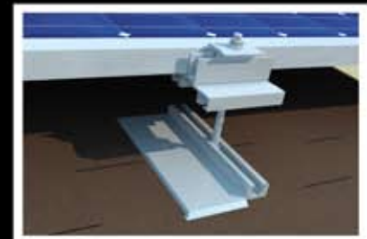
BOND PANEL WITH TOP CLAMP
